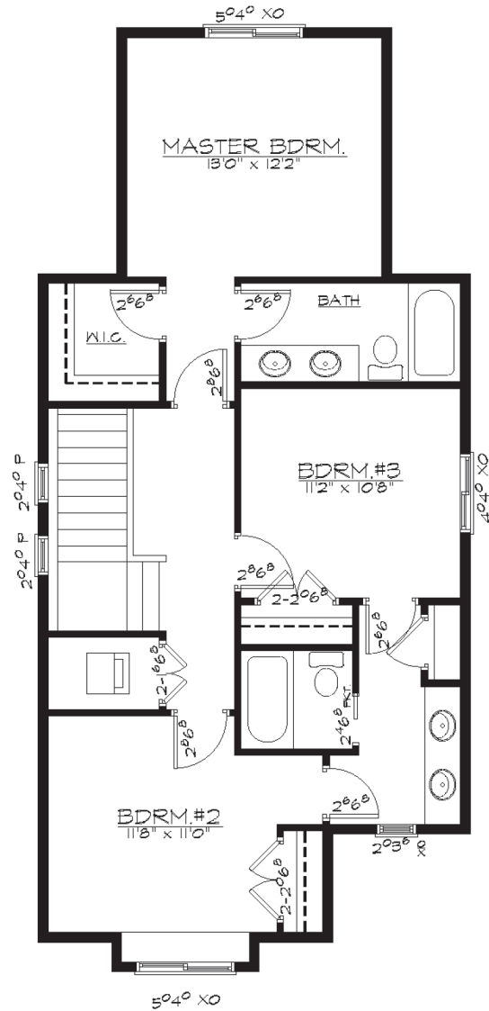
UPPER FLOOR PLAN 'A' FINISHED AREA = 828 SQ. FT. (8' CEILING)
