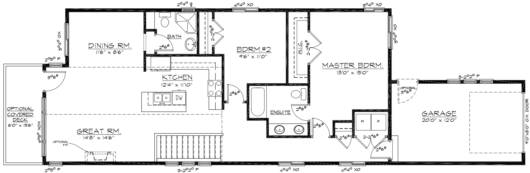
2 Bedroom Main Central Kitchen
